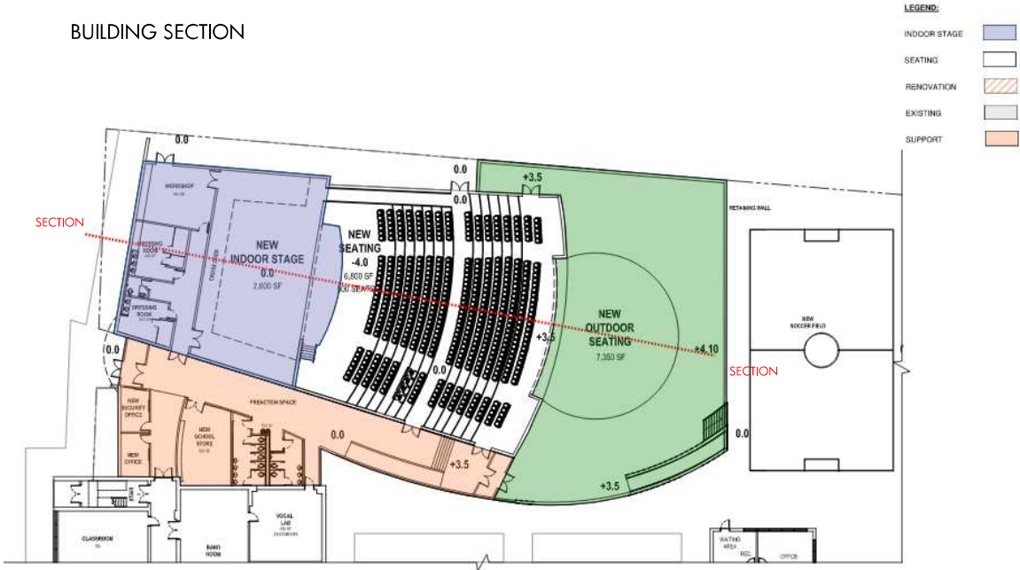
PARTIAL PLAN
