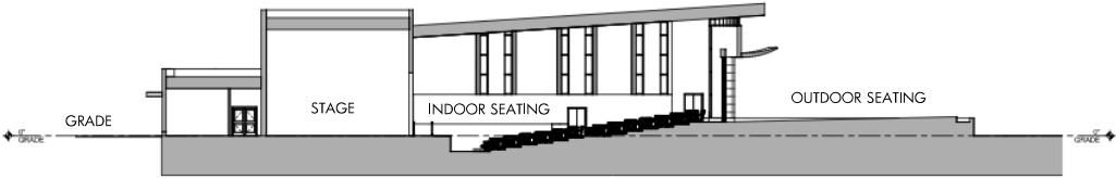
BUILDING SECTION
